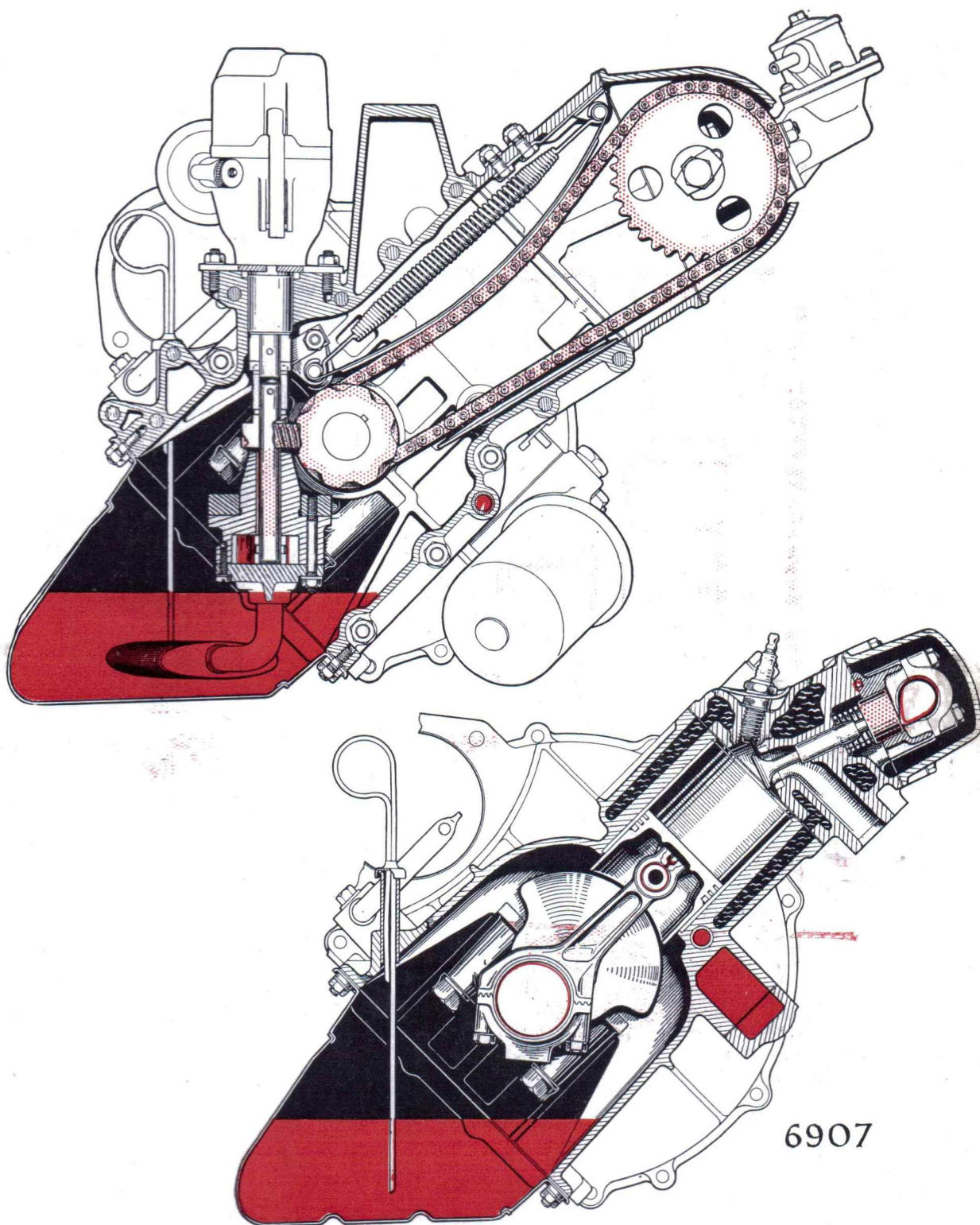
Fig. 2. Engine—cross sections
