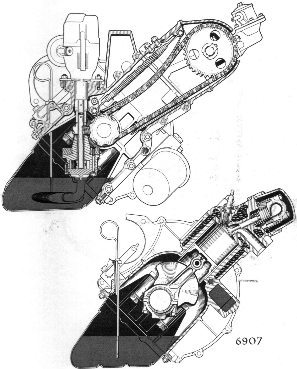
Fig. 2. Engine—cross sections
