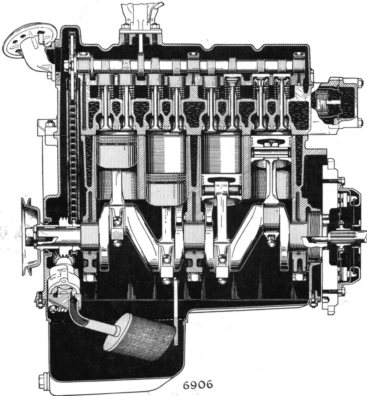
Fig. 1. Engine—longitudinal section
