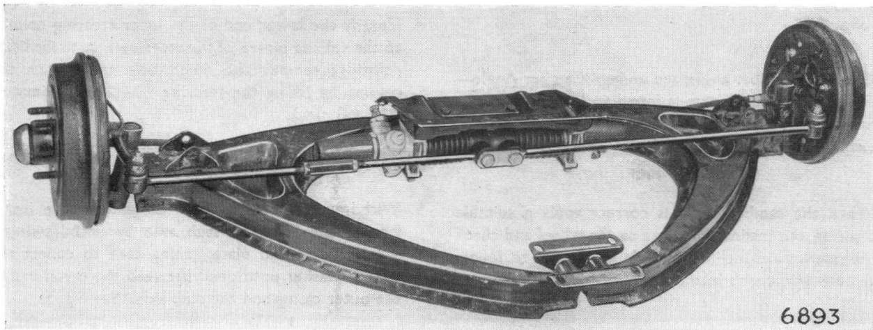
Fig. 3. The front suspension assembly removed from the car
