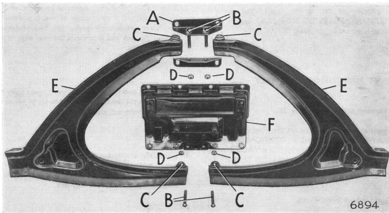
Fig. 4. Exploded view of front suspension wishbones and brackets
