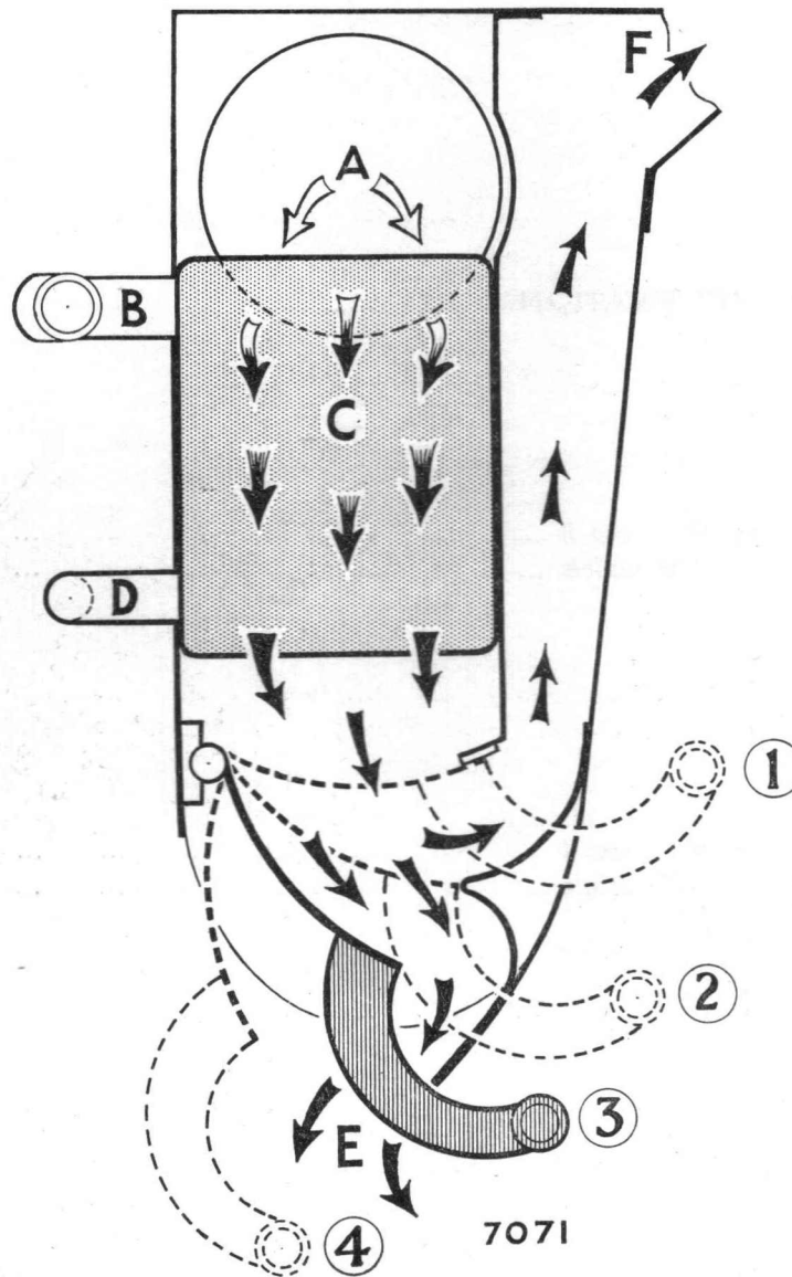
Fig. 1. Schematic section of heater
